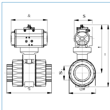
VALVE WITH SINGLE ACTING ACTUATOR
